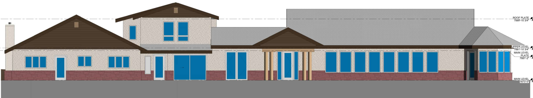
2 NORTH ELEVATION - PROPOSED 1/4" = 1'-0"
