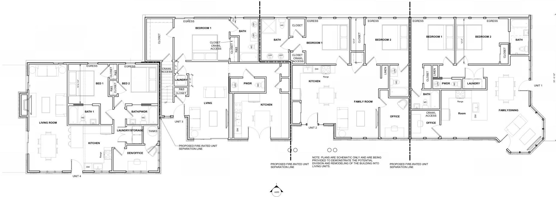
2 MAIN LEVEL - PROPOSED 1/4" = 1'-0"
